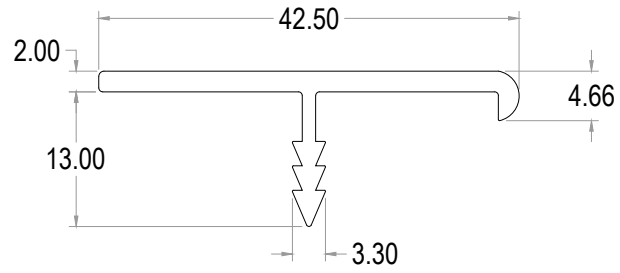
END VIEW
