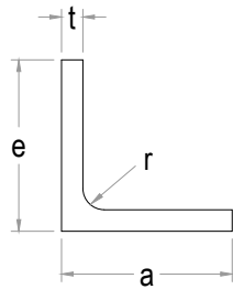
END VIEW
